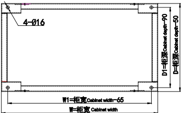
FS柜活动底座示意（固定同） Activities indicate the base FS cabinet (fixed with)
