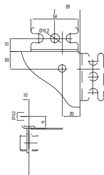
ME02墙壁挂件 / ME02 wall mounting parts
